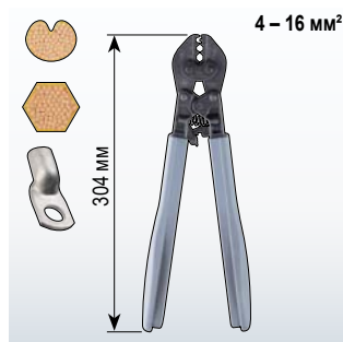
CRIMPFOX-RCT 16-1 1212731
