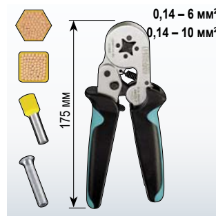
CRIMPFOX 6H 0,14–6 mm² 1212046
