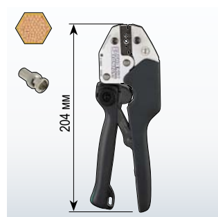
CRIMPFOX-CX 4,52-M 1212713
